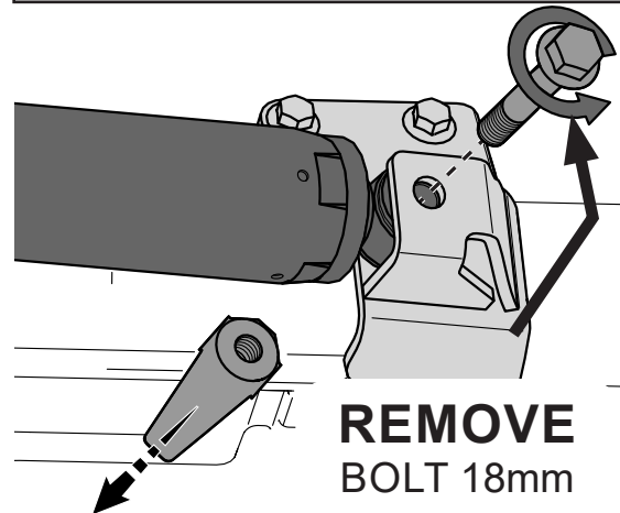
JK/JL/JT FALCON TRACK BAR BOLT MOUNT
