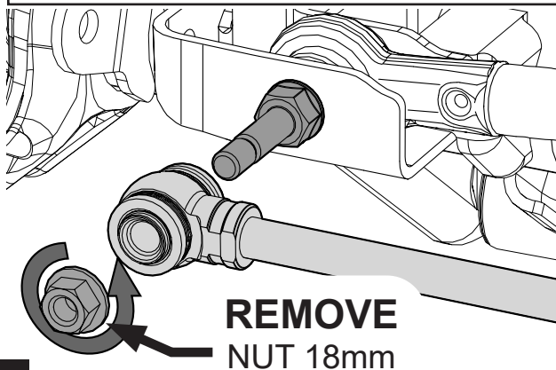
JK/JL/JT FALCON TRACK BAR STUD MOUNT
