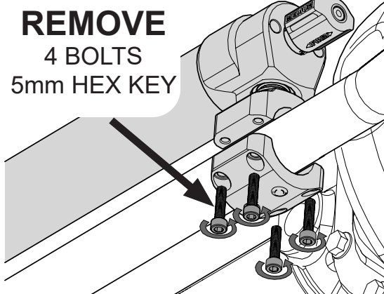
JK/JL/JT FALCON TIE ROD TUBE CLAMP MOUNT
